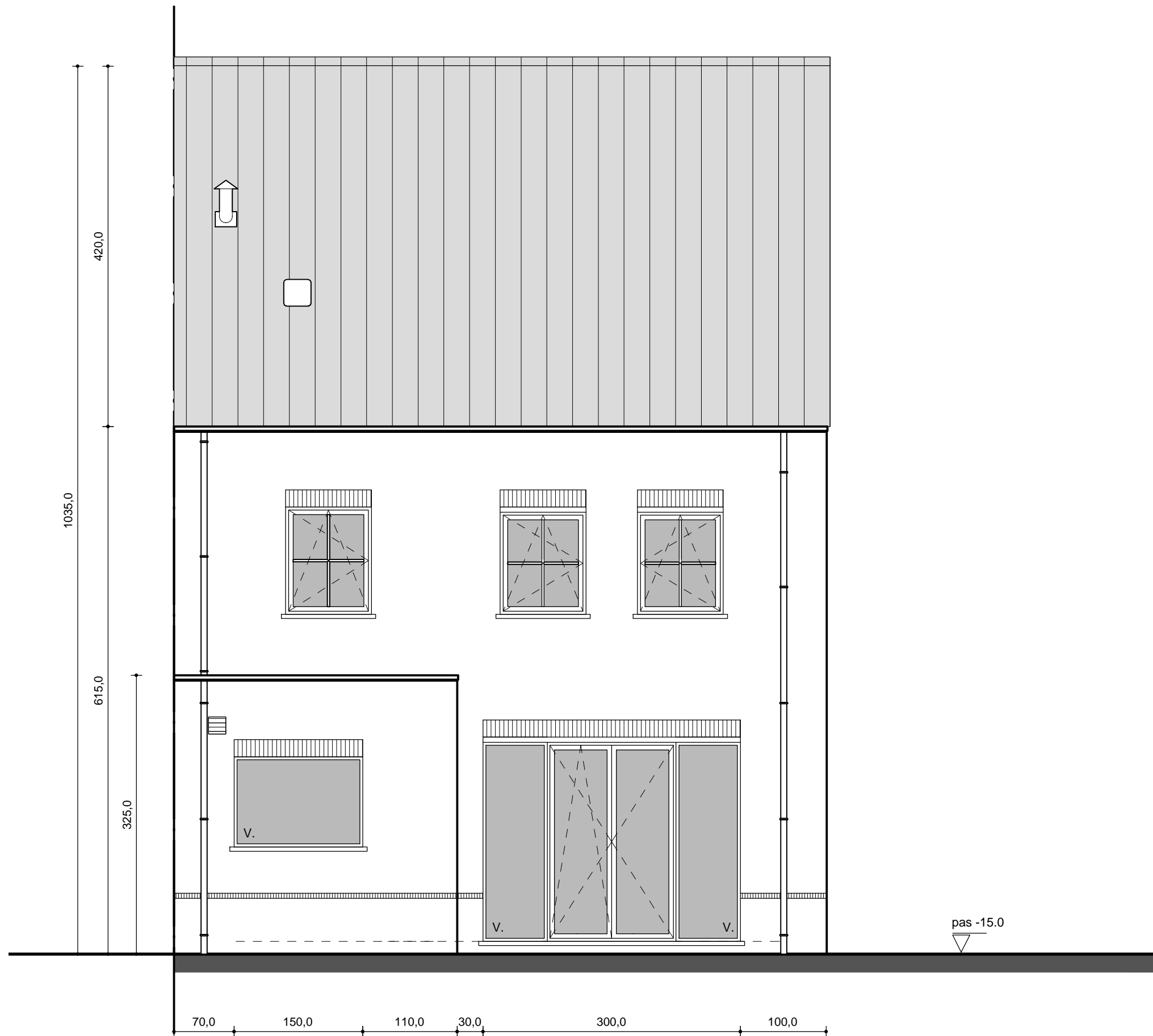
ACHTERGEVEL (D.D)
